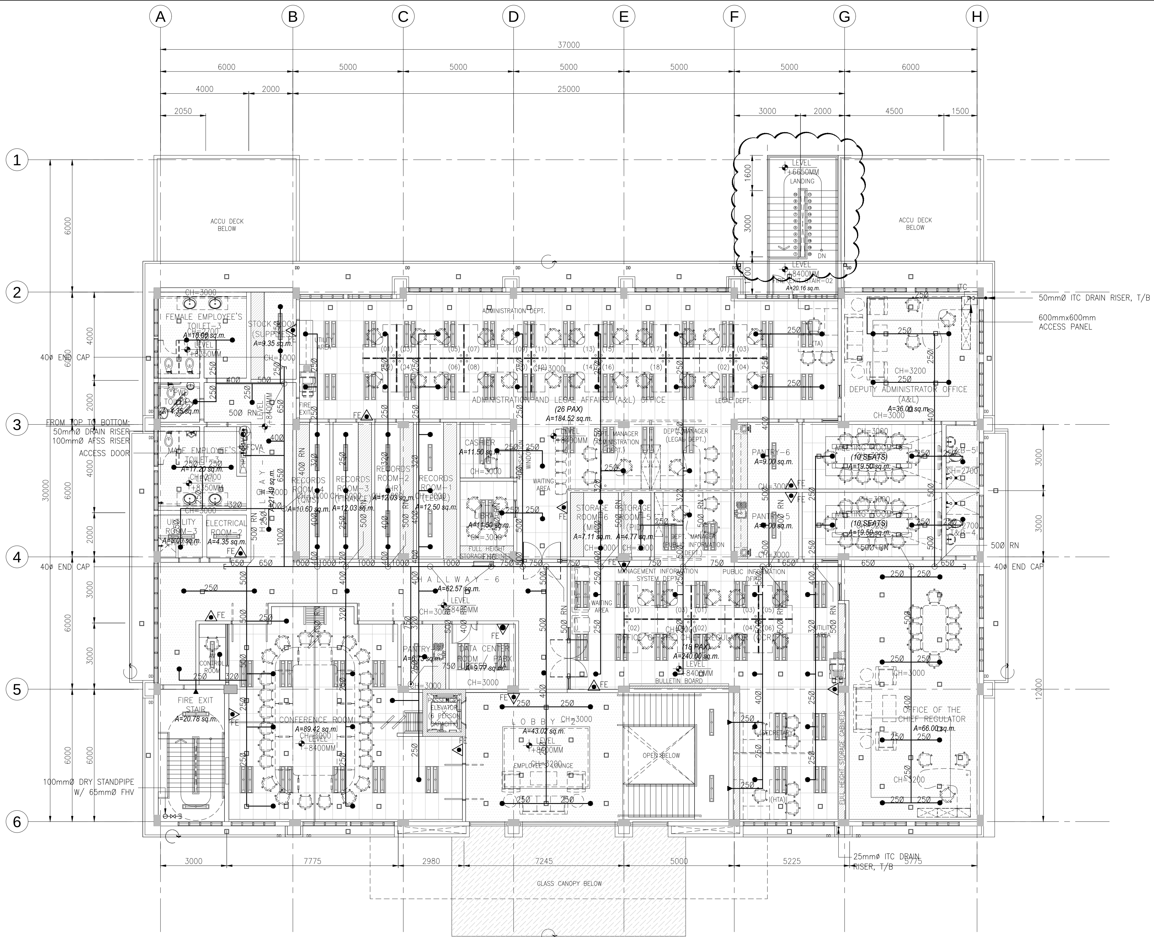
I THIRD FLOOR FIRE PROTECTION LAYOUT F-0103 SCALE 1:100M
