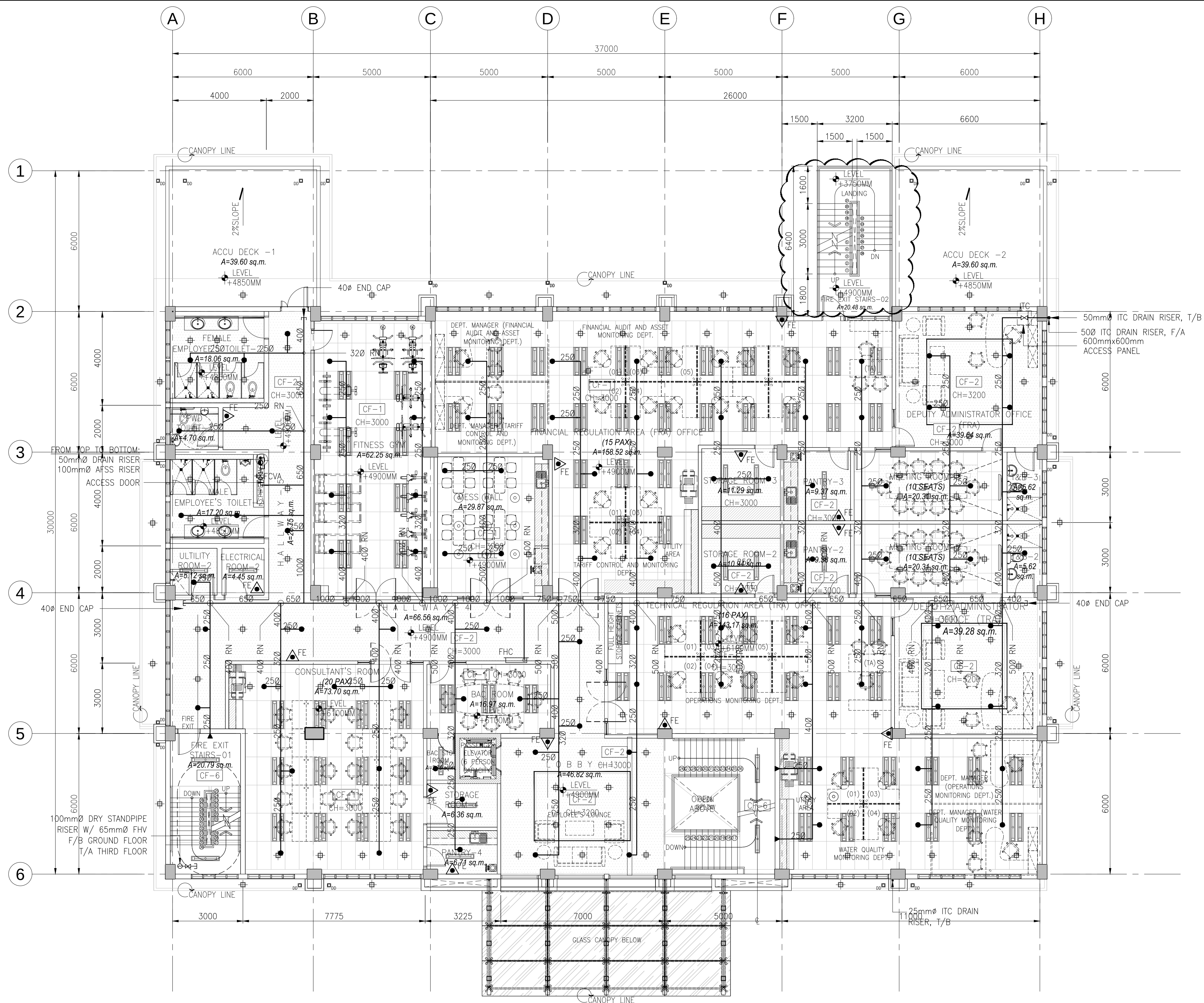
I SECOND FLOOR FIRE PROTECTION LAYOUT F-0102 SCALE 1:100M
